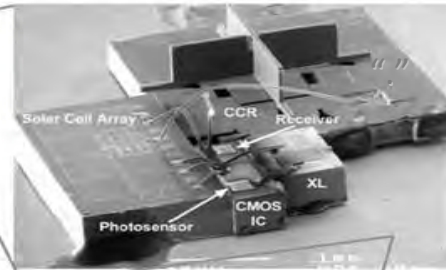
Smartdust wireless sensor (2002)
